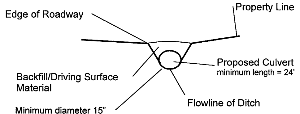
End View
